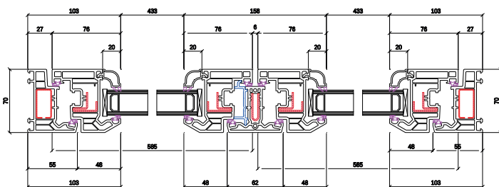
HORIZONTAL CROSS SECTION - 62MM INVISIBLE MULLION (IDENTICAL FOR CASEMENT AND FRENCH CASEMENT)
