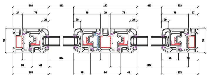
HORIZONTAL CROSS SECTION - 84MM VISIBLE MULLION (IDENTICAL FOR CASEMENT AND FRENCH CASEMENT)
