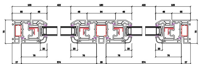
HORIZONTAL CROSS SECTION - 84MM VISIBLE MULLION (IDENTICAL FOR CASEMENT AND FRENCH CASEMENT)
