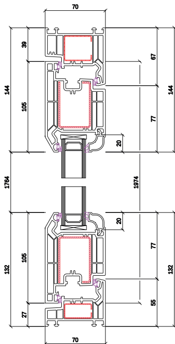
OPEN OUT DOOR WITH 55MM THRESHOLD
