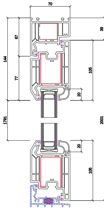
OPEN IN DOOR WITH 39MM THRESHOLD
