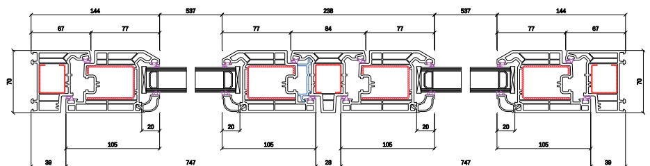
FRENCH DOOR OPEN IN CROSS SECTION WITH 84MM FLOATING MULLION
