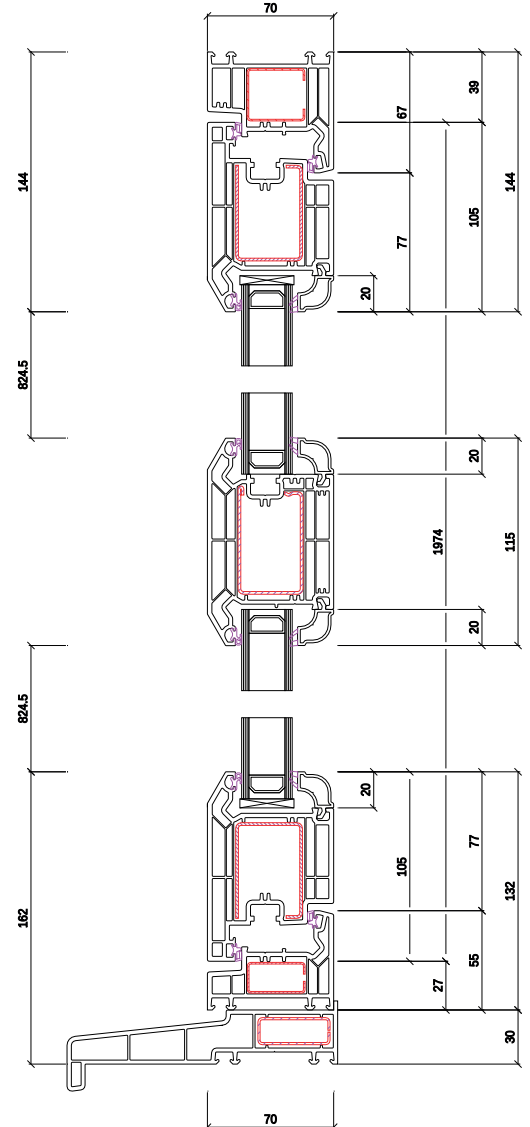
OPEN OUT DOOR WITH 115MM MIDRAIL 55MM THRESHOLD AND 150MM CILL
