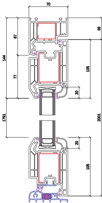
OPEN IN DOOR WITH 19MM THRESHOLD
