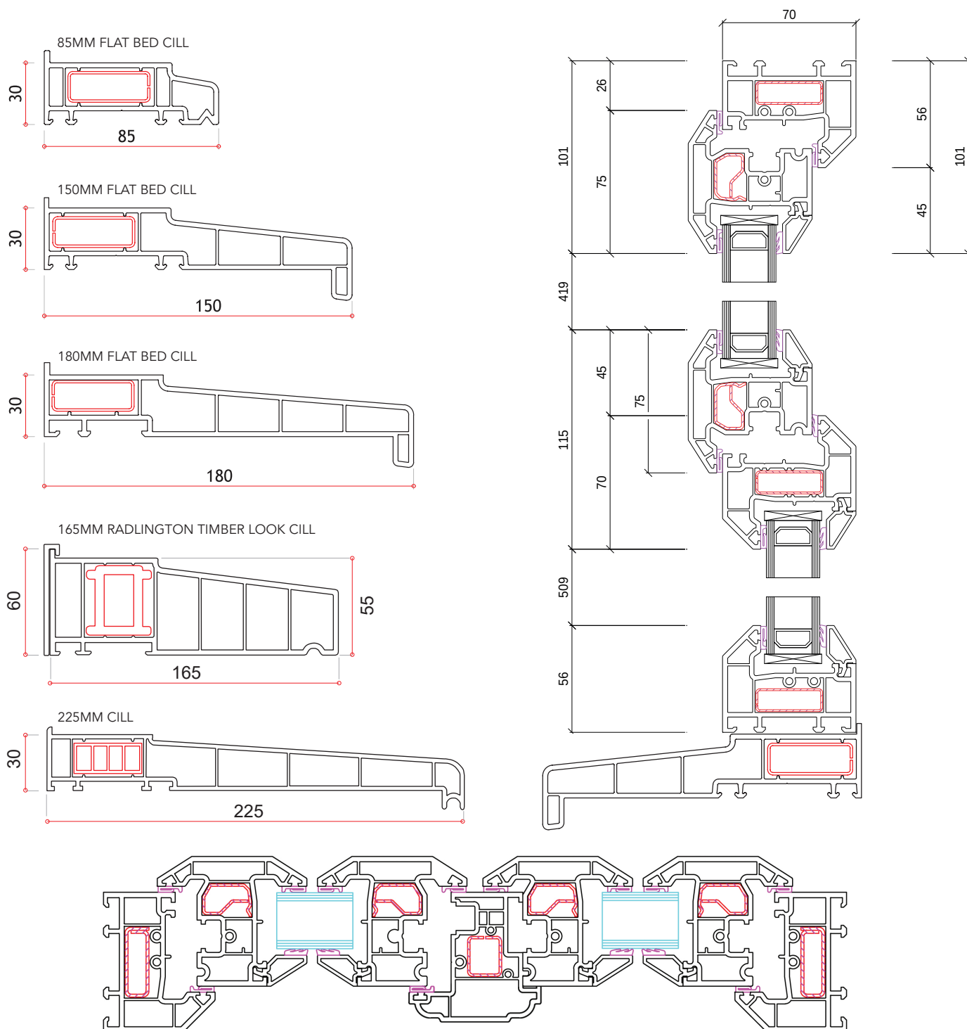
FRENCH WINDOW HORIZONTAL CROSS SECTION
