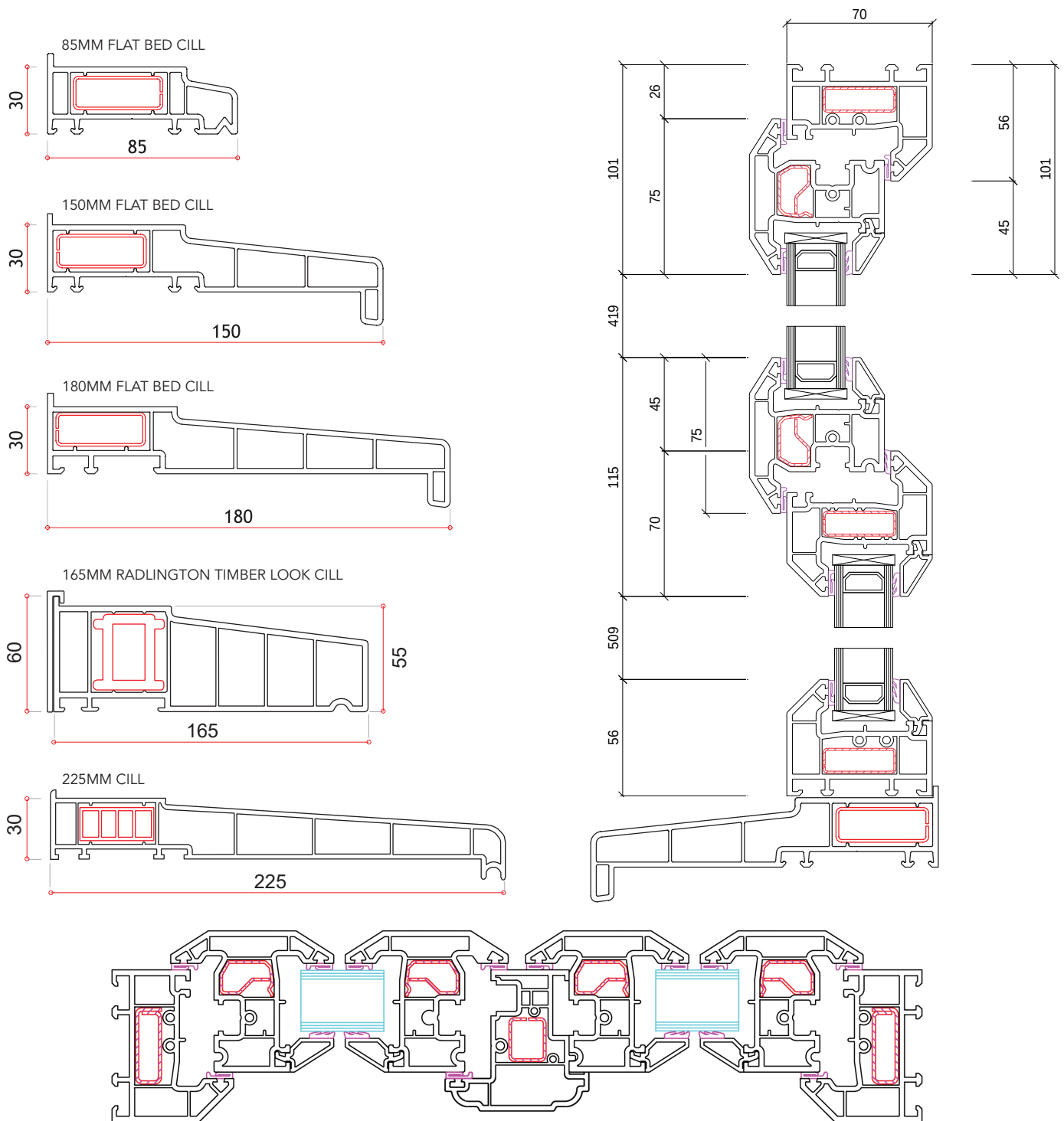
FRENCH WINDOW HORIZONTAL CROSS SECTION
