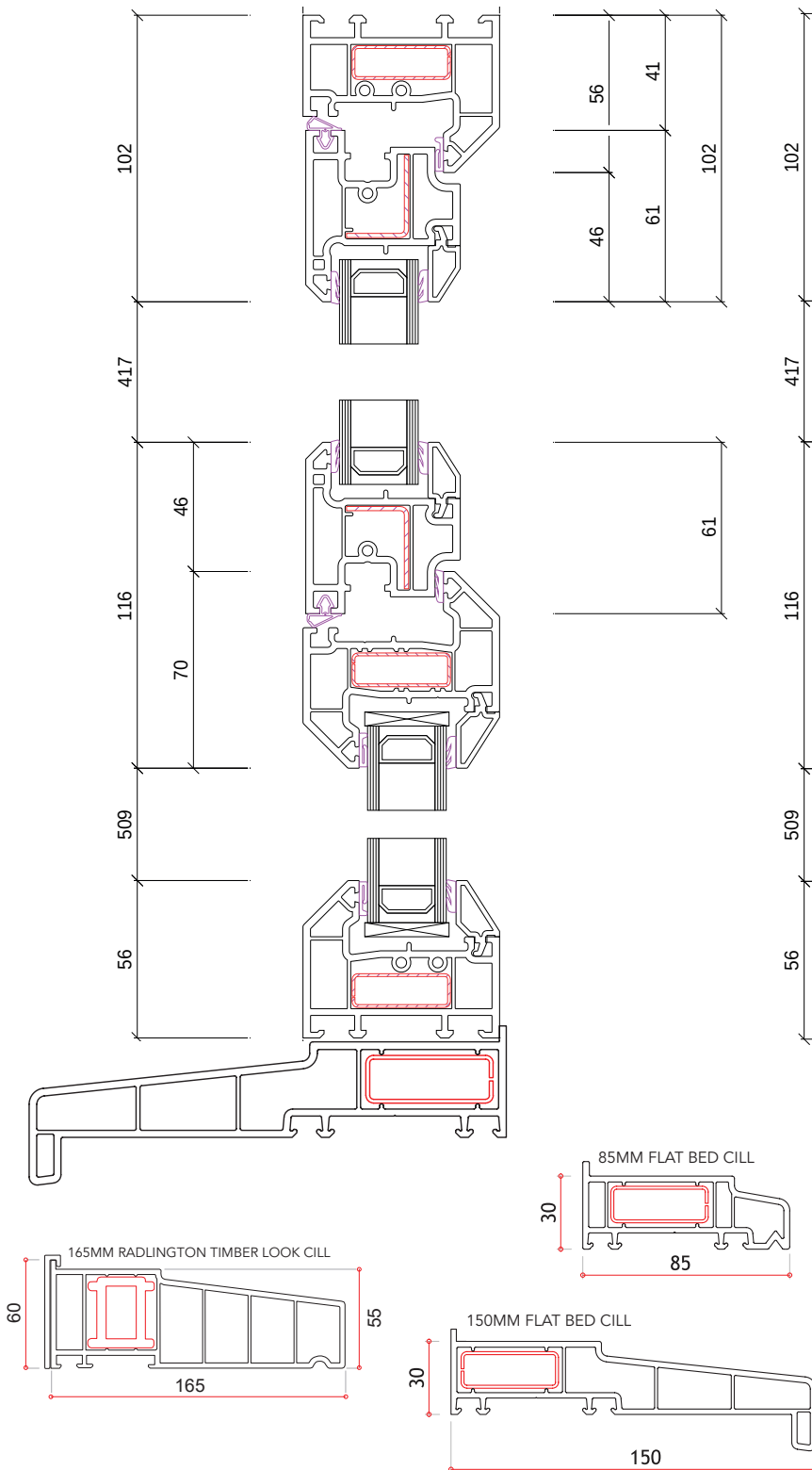
System 10 Flush Sash (bevelled)
