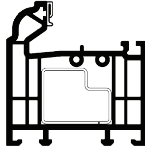
72MM PVC-U THRESHOLD (OVOLO)
